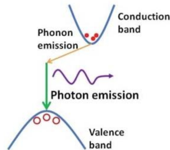
Indirect bandgap
