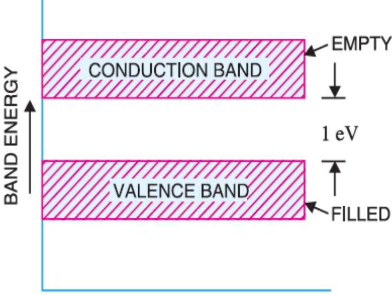
Semiconductors
